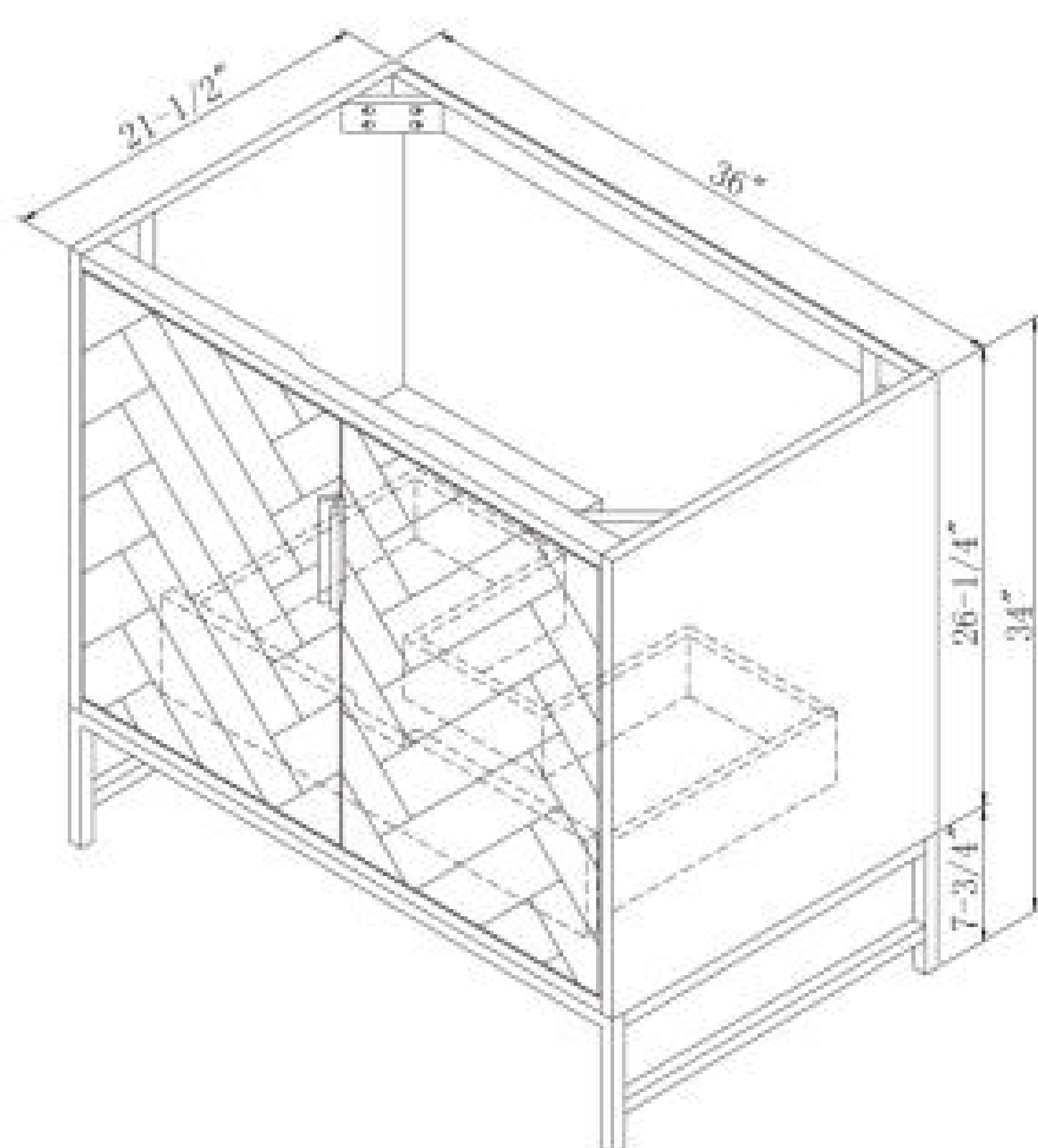
QN3621D Vanity 2 x Door / 1 x Drawer
