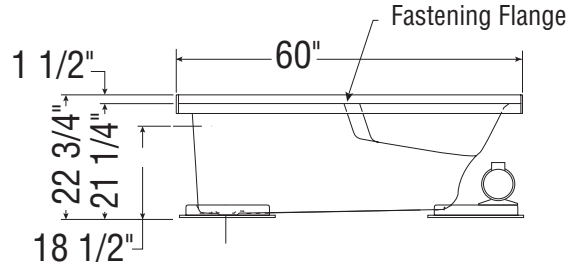
10-jet Bodywrap System SBF-3660L BWS (illustrated)
